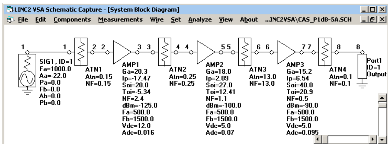
Figure 3, LINC2 VSA System Schematic
