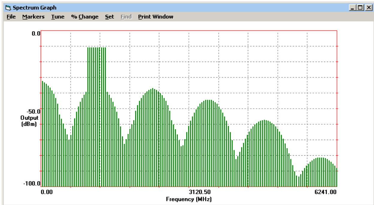
Figure 2, LINC2 VSA Spectrum Analysis Plot
