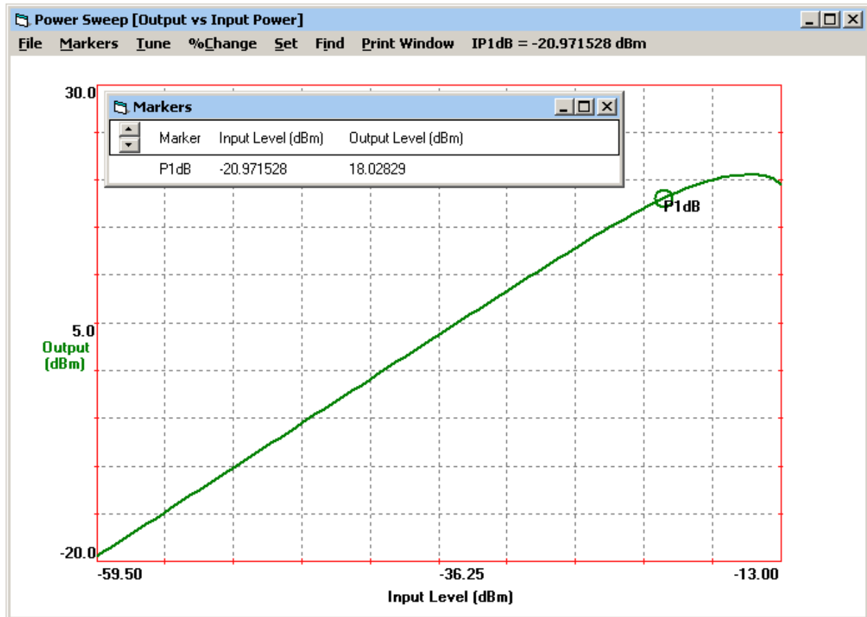
Figure 4, LINC2 VSA Power Sweep Plot
