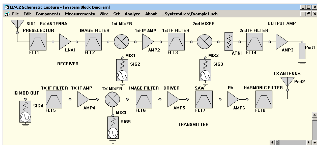
Figure 1, LINC2 VSA Block Diagram
